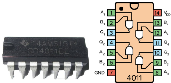
CD4011BE IC GATE NAND 4CH 2-INP 14DIP
